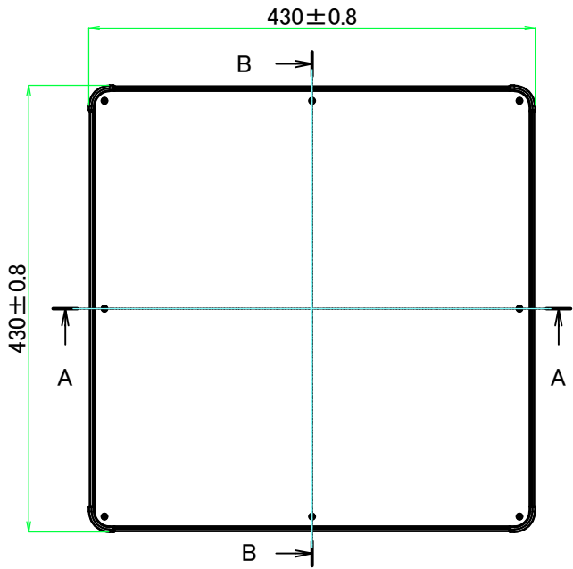
E view
